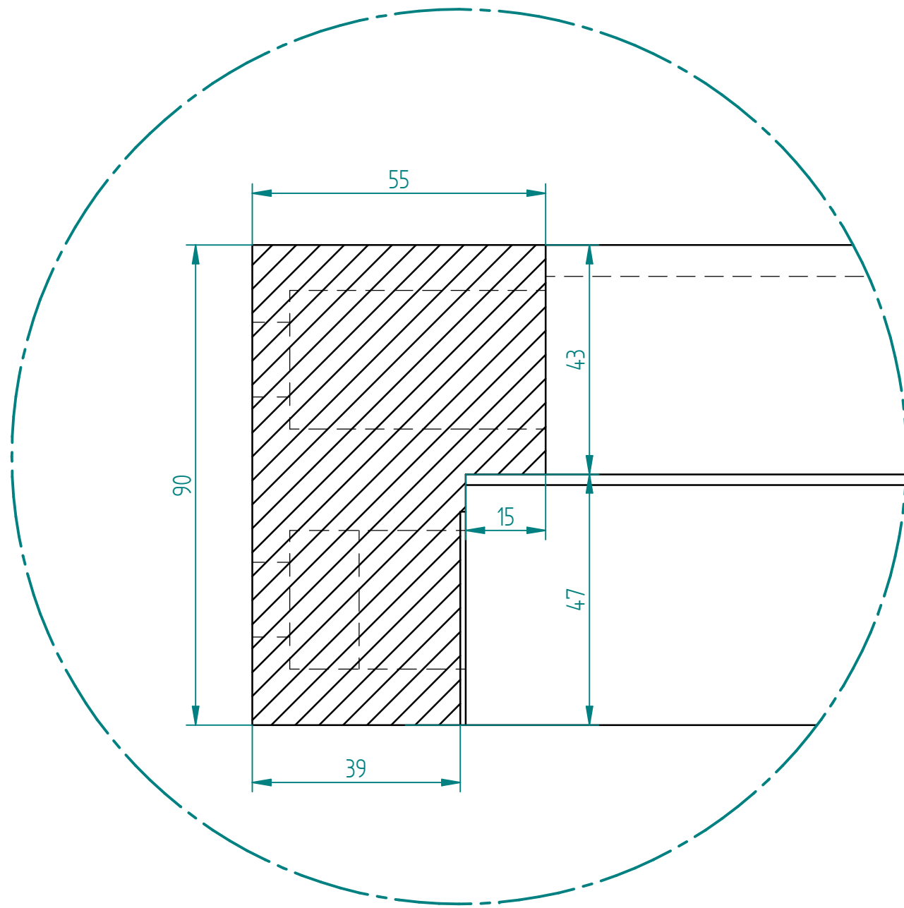
DETAIL B
